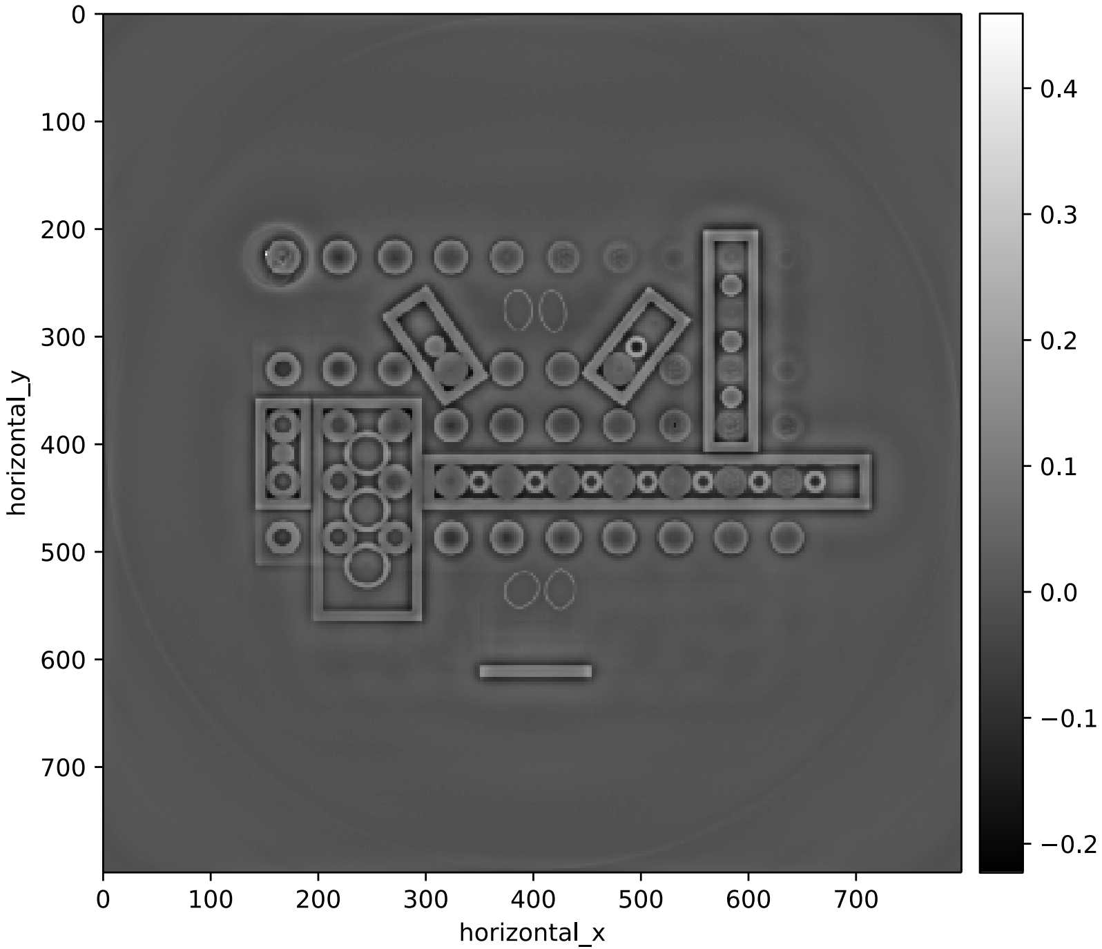
CGLS reconstruction
