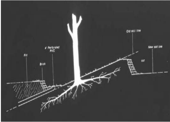
Figure 6 - Side view showing proper method of raising and lowering the grade around trees.
