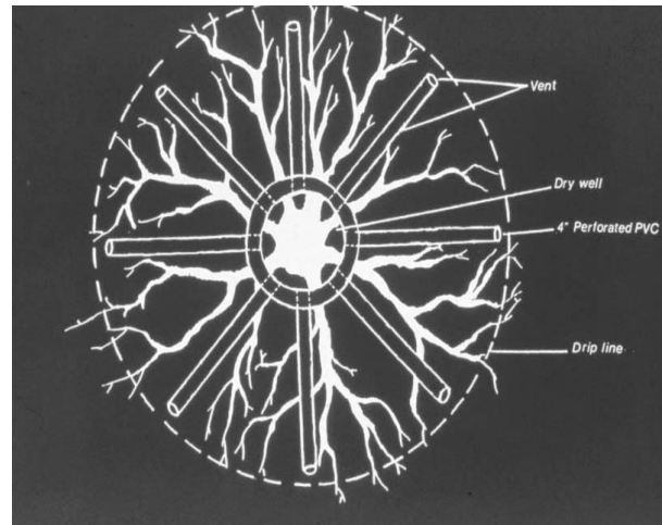
Figure 4 - Top view showing proper construction of well and drainage system for use around trees where soil fill has been added to raise grade.
