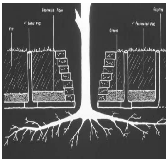
Figure 3 - Side view showing proper construction of well and drainage system for use around trees where soil fill has been added to raise grade.
