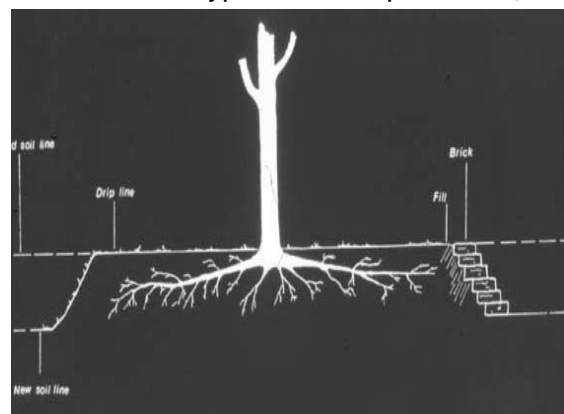
Figure 5 – Side view showing proper method of lowering grade near trees.
