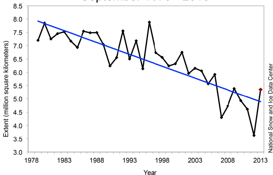
FIGURE 2.13 The time series of September Arctic sea ice extent from 1979-2013. SOURCE: National Snow and Ice Data Center, http://nsidc.org/arcticseaicenews .
