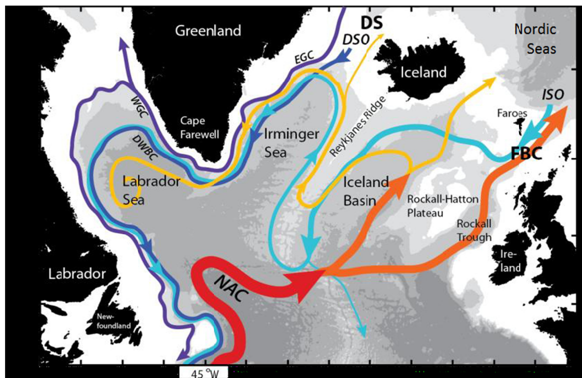
FIGURE 2.1 Schematic of the major warm (red to yellow) and cold (blue to purple) water pathways in the North Atlantic subpolar gyre. Acronyms not in the text: Denmark Strait (DS); Faro Bank Channel (FBC); East and West Greenland Currents (EGC, WGC); North Atlantic Current (NAC); DSO (Denmark Straits Overflow); ISO (Iceland-Scotland Overflow). Figure courtesy of H. Furey (WHOI).
