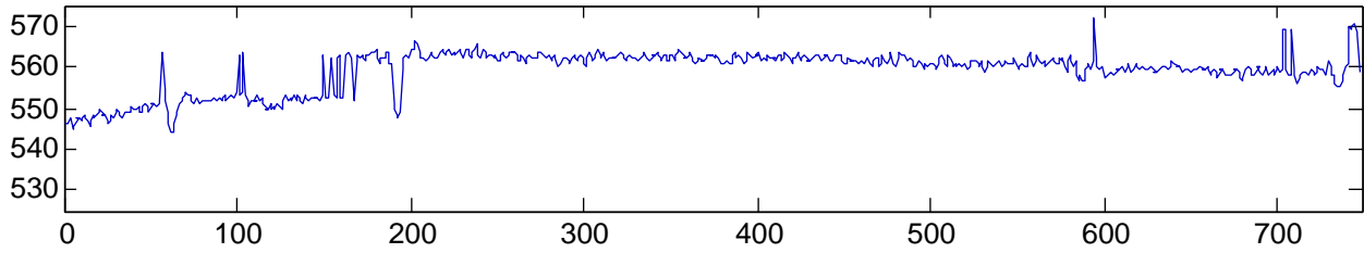
slice timing + realign & unwarp (with fieldmap vdm)
