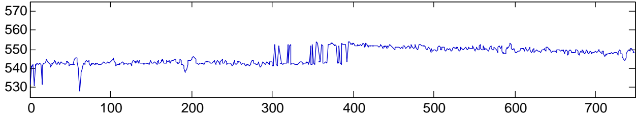
slice timing
