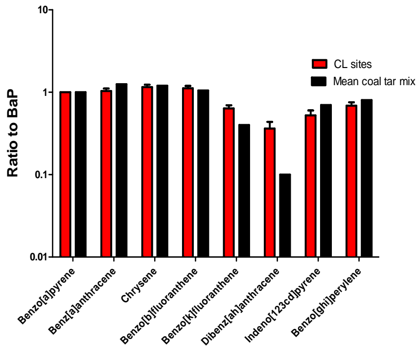
Figure 1. The mean ratio of PAH to BaP in the soil from potentially contaminated sites compared with coal tar mix.
