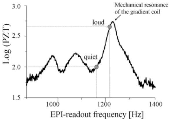
FIG. 2. Frequency response curve showing the amplitude of vibrations as a function of the EPI readout z-gradient frequency. Fine adjustment ( <10\% ) of the acquisition bandwidth resulted in a four-fold (12 dB) increase of the vibration amplitude from quiet to loud EPI protocols.
