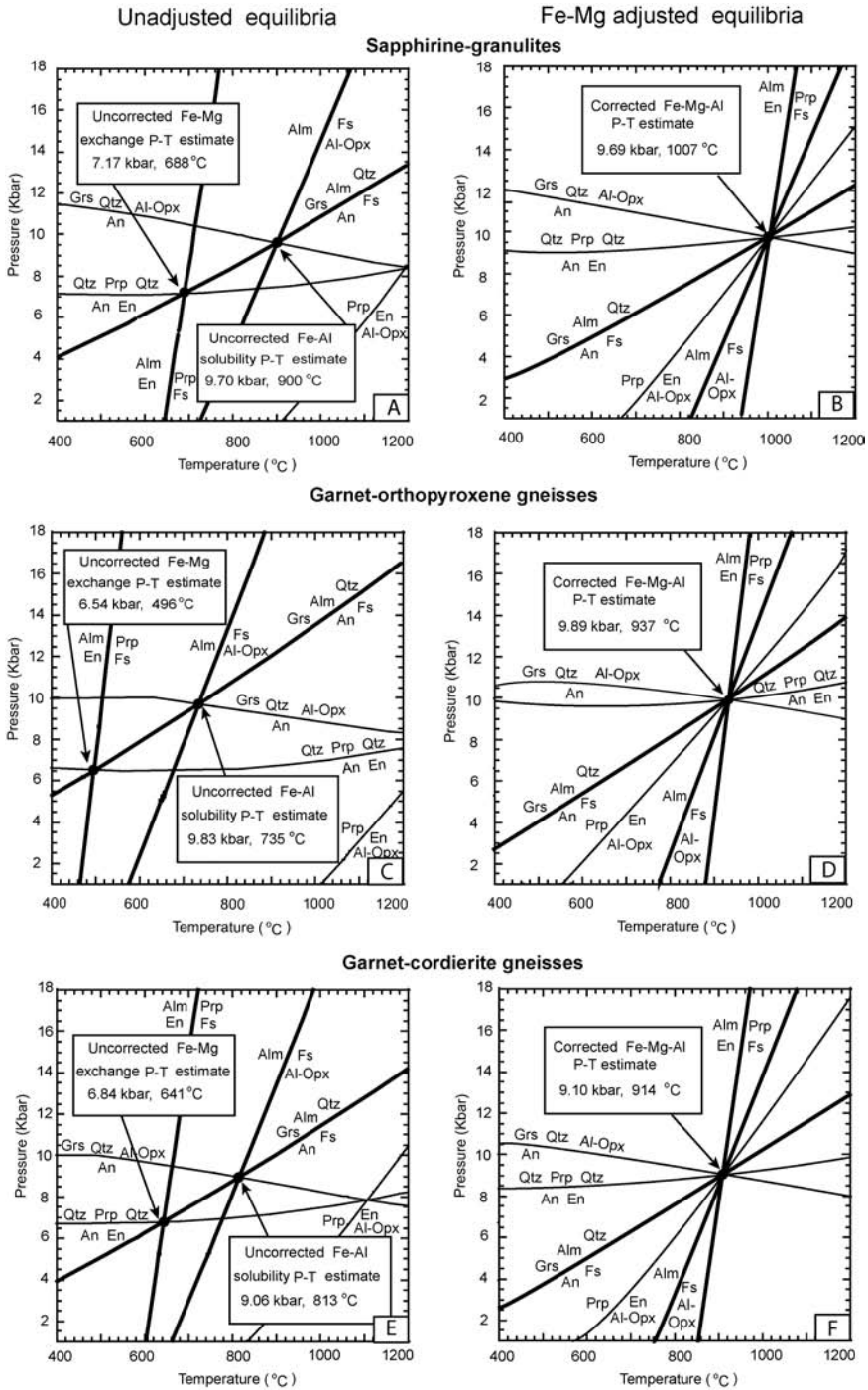
FIG. 6. P-T plots showing the convergence method of retrieval of the thermal peak conditions. A, C., and E display the typical spread in equilibria without adjustment of the mineral compositions. Of the six equilibria shown, only three are independent, and these are indicated in bold. B, D, and F show intersection of the curves of the mineral equilibria through adjustment of Fe-Mg ratios of garnet and orthopyroxene according to mass balance constraints so that all equilibria intersect at a point. See text for details.
