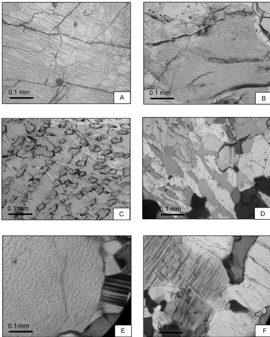
FIG. 2. Photomicrographs showing textures of exsolved feldspar in granulites from the Palni Hills. A and B. Photomicrographs showing mesoperthites in sapphirine-bearing granulites. C and D. Antiperthitic plagioclase containing exsolved rods of K-feldspar in garnet-orthopyroxene-bearing gneisses. Antiperthitic plagioclase grains containing exsolved patches of K-feldspar are elongated and parallel. E. Perthitic alkali feldspar with plagioclase in charnockites. F. Antiperthite with alkali feldspar in charnockites.
