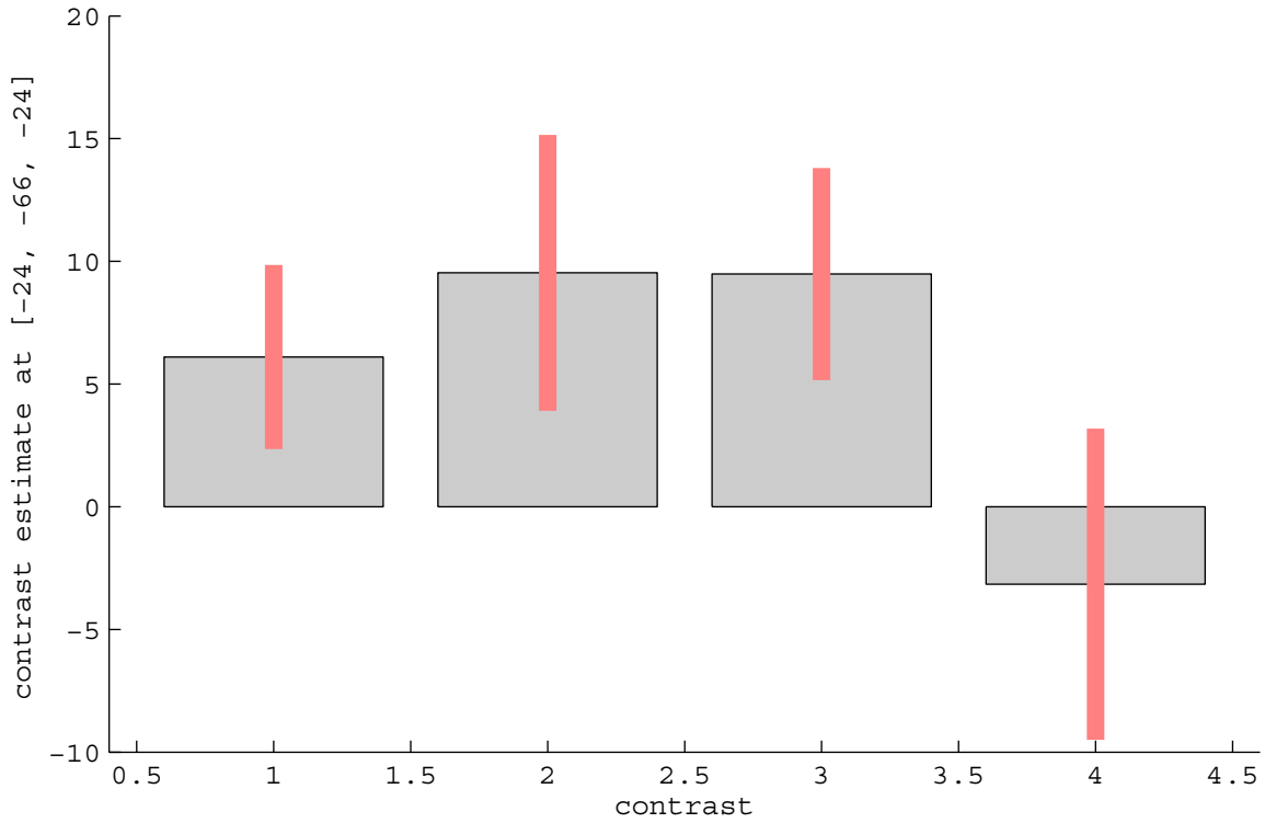
Contrast estimates and 90% C.I. effects of interest
