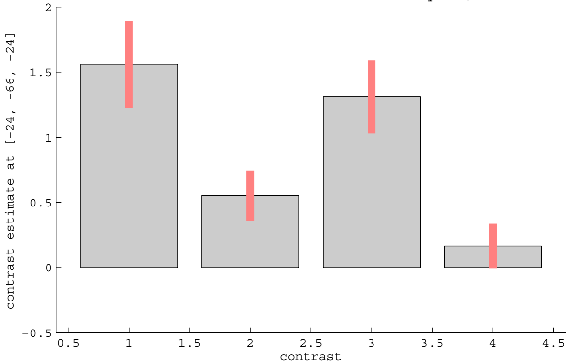
Contrast estimates and 90% C.I. Effects of interest 'eye(4,4)'
